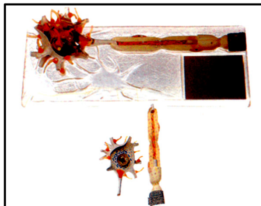
Neuron Model
